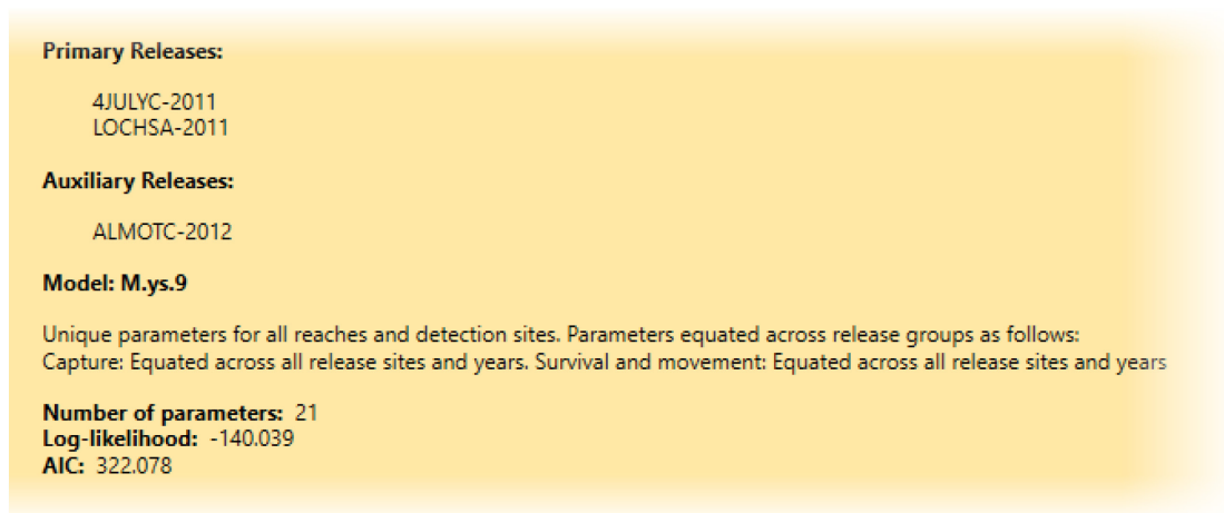
Figure 32. The header for all Model-Specific Reports.
