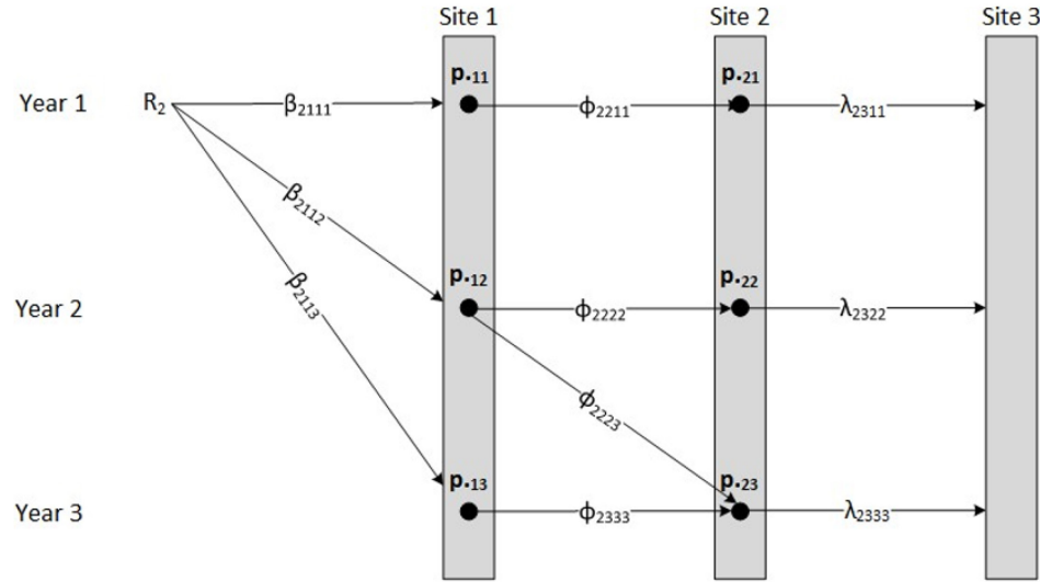
Figure 2. A graphical representation of Model M.y.s.4 with the capture parameters (in bold) equated across release sites.
