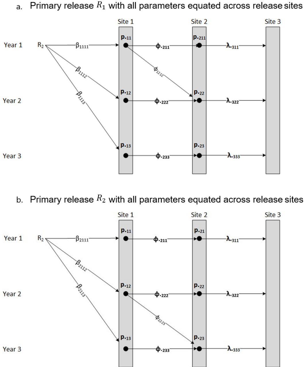
Figure 3. A graphical representation of Model M.y5 with all parameters equated across release sites. The equated parameters are in bold.
