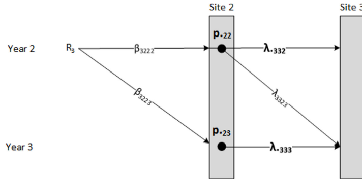
Figure 4. A graphical representation of Model M.y9 with all parameters shared by releases R_1 , R_2 , and R_3 and equated across all releases. The equated parameters are in bold.
