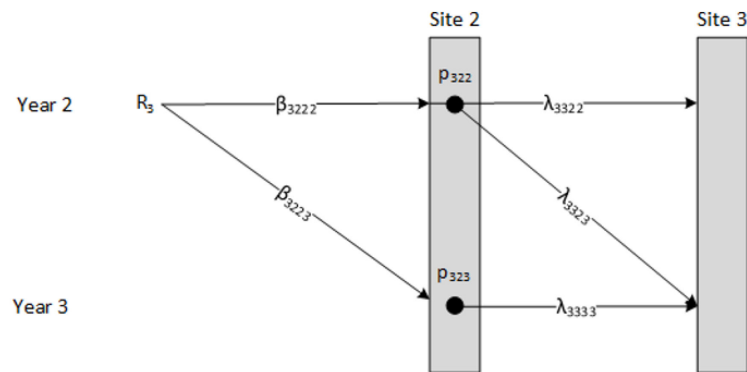
Figure 1. A graphical representation of Model M.y.s.1 with no shared parameters for a hypothetical study.
